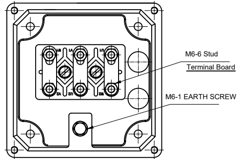
TERMINAL BOX DETAILS
