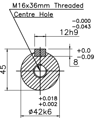
EXTENSION DETAILS
