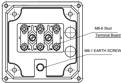
TERMINAL BOX DETAILS
