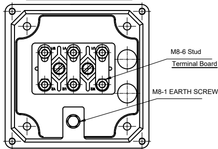
TERMINAL BOX DETAILS
