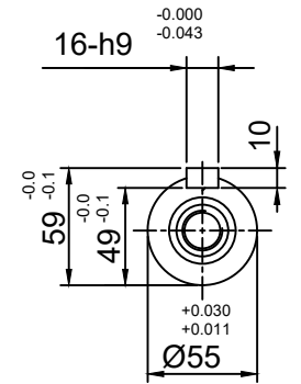
EXTENSION DETAILS
