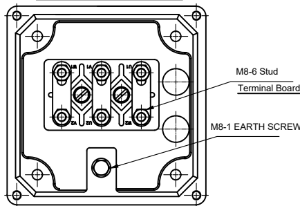
TERMINAL BOX DETAILS
