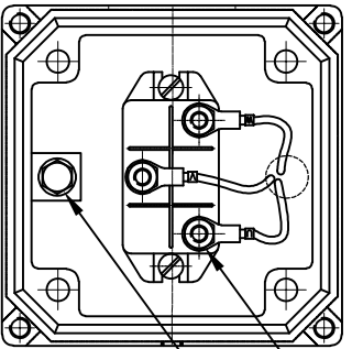
TERMINAL BOX DETAILS
