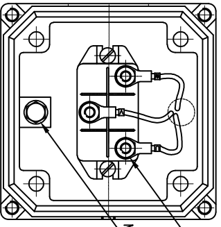
TERMINAL BOX DETAILS
