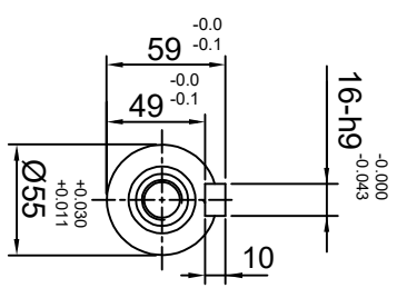
EXTENSION DETAILS
