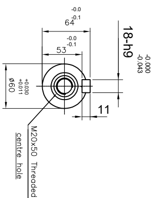
EXTENSION DETAILS
