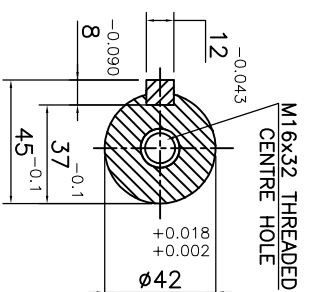
SHAFT EXTENSION DETAIL AT DRIVE END
